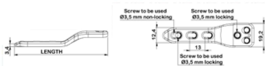
3.5 mm Pediatric Locking Plate 110°
