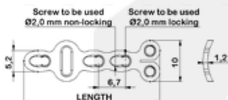
2.0 mm Mini Rotation Correction Locking Plate ( 2 Holes Head )
