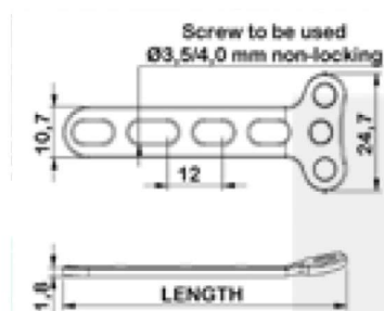
3.5 mm T - Plate Right - Angled ( 3 Holes On Head )
