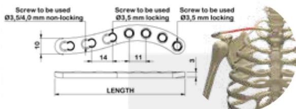
3.5 mm Clavicle Locking Compression Plate
