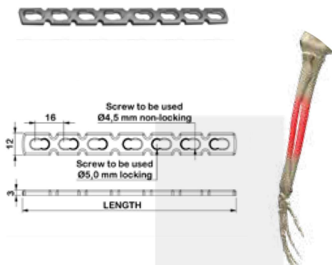
4.0 / 4.5 / 5.0 mm Reconstruction Locking Compression Plate
