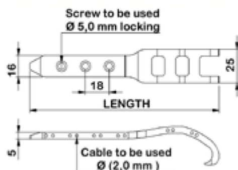
4.5 / 5.0 mm Trochanteric Cable Hook Plate 2
