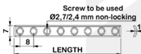
Quarter 1 / 4 Tubular Plate
