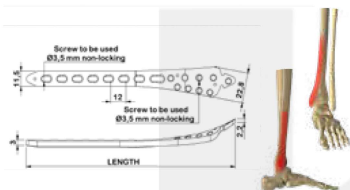
3.5 mm Distal Medial Plate 2
