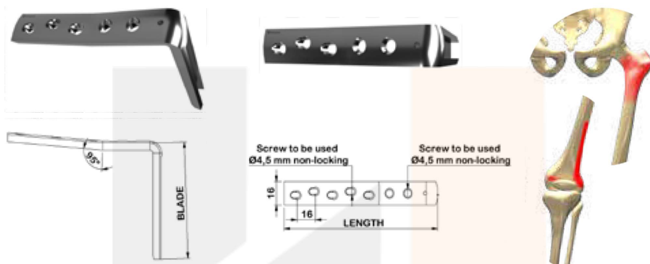
4.5 mm 95° Angled Blade Plate for Operation on Adult Femur
