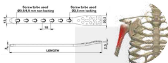
3.5 mm Proximal Humerus Locking Compression Plate 3
