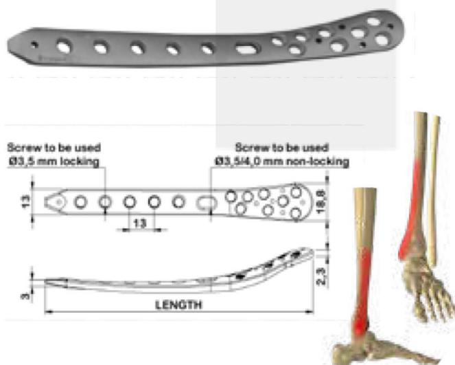
3.5 / 4.0 mm Distal Medial Tibia Locking Compression Plate 1
