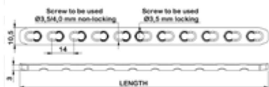
3.5 mm Locking Compression Plate
