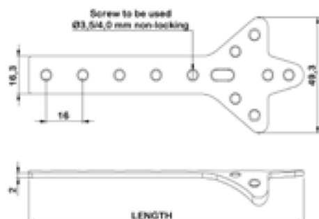
3.5 mm Cloverleaf Plate
