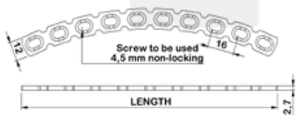
4.5 / 6.5 mm Narrow Compression Plate
