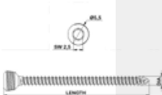
2.7 mm Locking Screw ( 5.5 mm Head DIA. )
