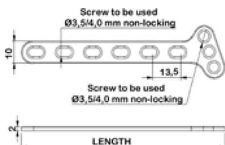
3.5 mm Compression T - Plate Oblique - Angled
