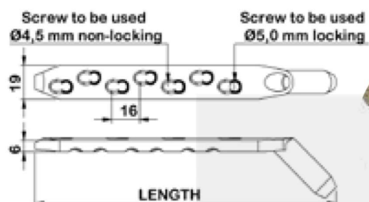
DHS Locking Plate 135°
