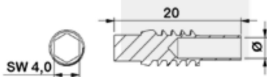
Elastic Nail End Cap
