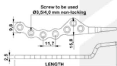
3.5 mm Clavicle Hook Plate
