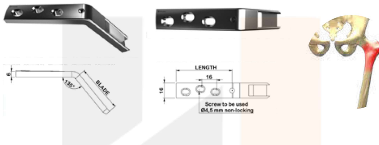
4.5 mm 135° Angled Blade Plate for Operation on Adult Femur
