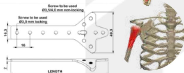
3.5 mm CloverLeaf Locking Plate
