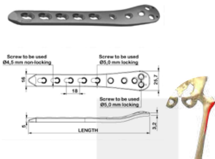
4.5 / 5.0 mm Proximal Femur Locking Compression Plate 1
