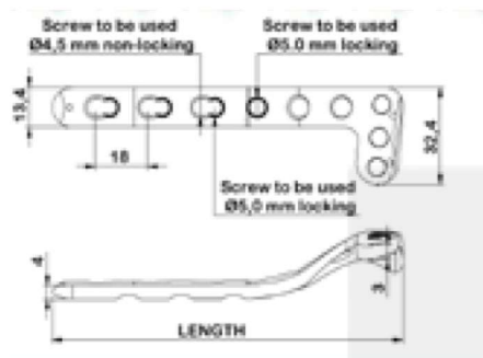
4.5 / 5.0 mm Proximal Lateral Tibia Locking Plate 2
