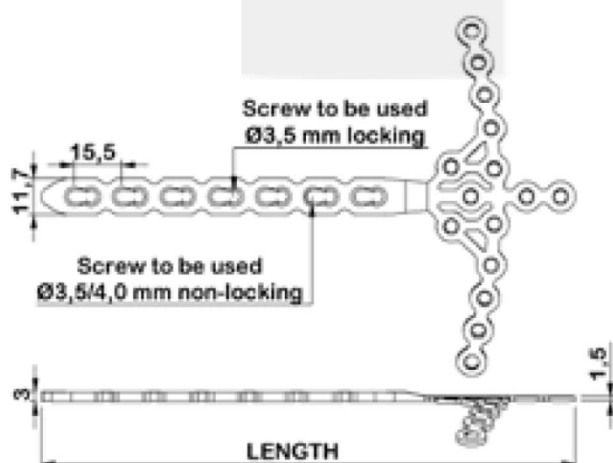
3.5 / 4.0 mm Distal Tibia Locking Pilio Plate
