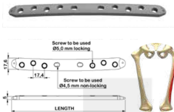
4.5 / 5.0 mm Locking Plate Broad Curved
