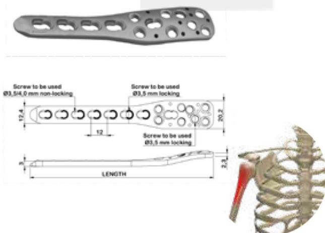
3.5 mm Proximal Humerus Locking Compression Plate 2
